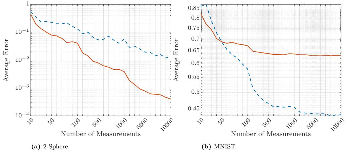
Fig. 5: Comparison of OMS (dashed, blue) and a modified version (solid, red) as described in (23).
