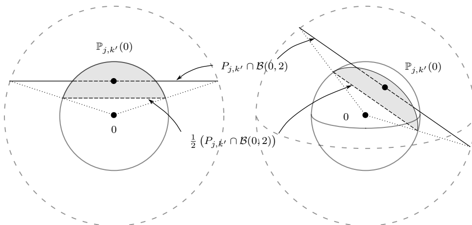
Fig. 3: Two views of an admissible set \text{conv}(\mathbb{P}_{\mathbb{S}}(P_{j,k'} \cap \mathcal{B}(\mathbf{0}, 2))) from (5) for a case with \|\mathbf{c}\|_2 = \|\mathbb{P}_{j,k'}(\mathbf{0})\|_2 < 1 .
