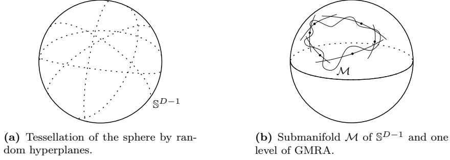
Fig. 1: One-bit measurements and GMRA.
