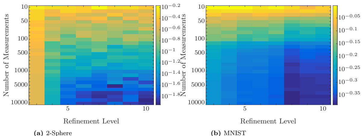
Fig. 7: Approximation error of OMS for different refinement levels j and numbers of measurements.
