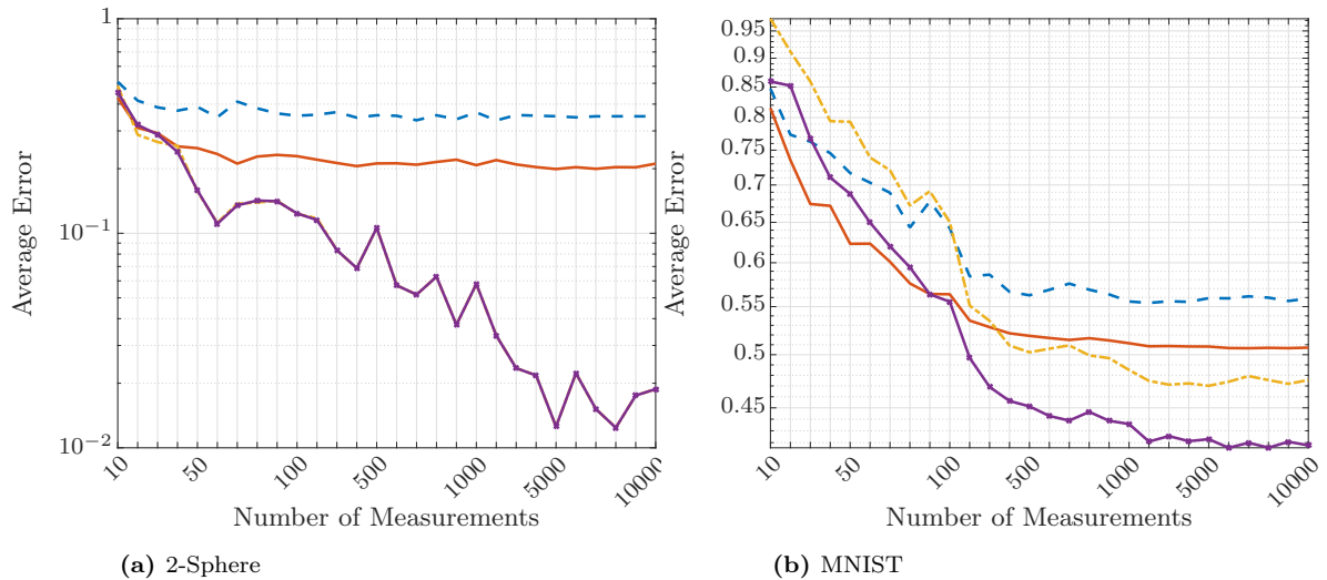
Fig. 6: Comparison of the following: Approximation by step I. of OMS when using tree structure (dashed, blue) and when comparing all centers (solid, red); approximation by step I.+II. of OMS when using tree structure (dashed with points, yellow) and when comparing all centers (solid with points, purple).
