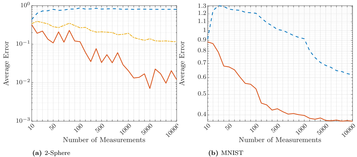
Fig. 4: Comparison of OMS-Simple for R = 1 (dotted-dashed, yellow), R = 1.5 (dashed, blue) and OMS (solid, red).
