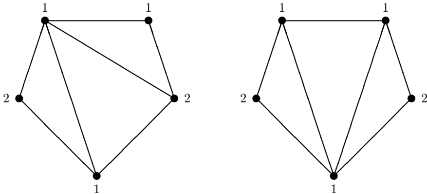
Figure 1: Two triangulations
