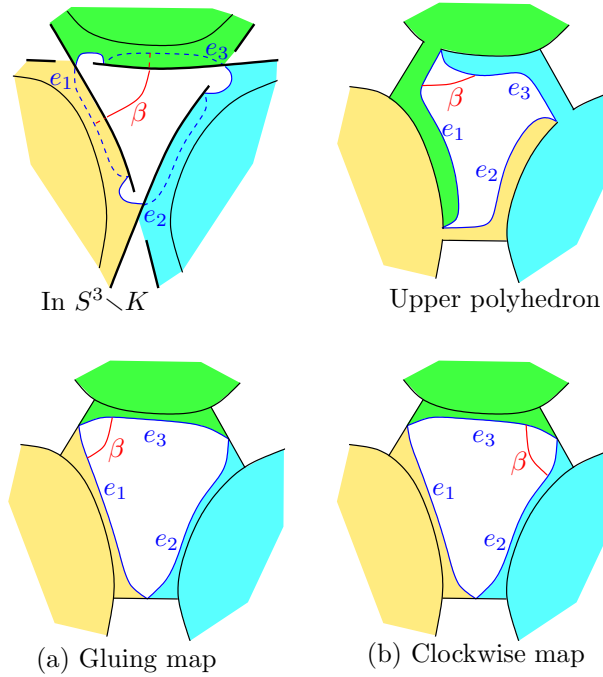
FIGURE 4.2. An example showing the image of an arc \beta under (a) the gluing map, and (b) the clockwise map.
