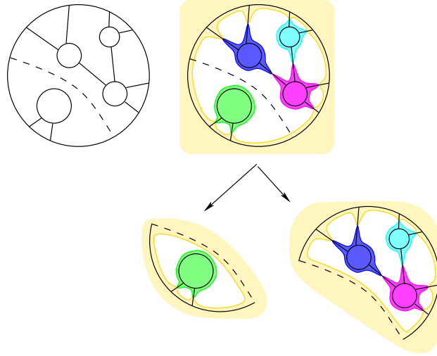
FIGURE 2.9. Splitting a lower polyhedron into two along a non-prime arc. These give two polyhedral regions, defined in Definition 3.10 on page 36.
