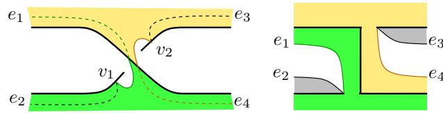
FIGURE 2.6. The shaded faces around the crossing of Figure 2.4
