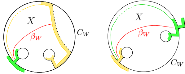
FIGURE 4.5. Regions R_W in the case \sigma_2 connects immediately to \beta_w .
