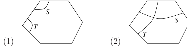
FIGURE 4.3. Cases (1) and (2) of Lemma 4.10 are illustrated for an example. Note if (2) happens, S and T intersect in two white faces.
