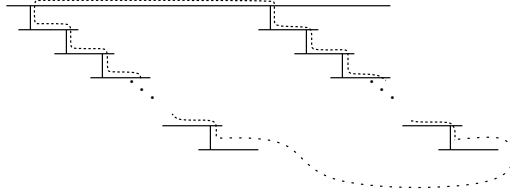
FIGURE 3.6. There exists a closed curve in H_A of the form of the dotted line above, where the arc with wider dots lies entirely on a white face, so does not intersect H_A nor any non-prime arcs of H_A .
