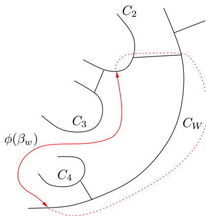
FIGURE 4.6. Image of \beta_w under clockwise map \phi: W \rightarrow W . Note there is an arc (dotted red) running through two state circles and a single segment of H_A connecting its endpoints. All red arcs shown form a normal trapezoid in the lower polyhedron
