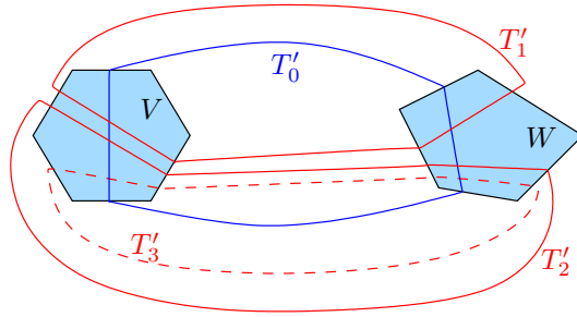
FIGURE 4.8. Normal squares in the lower polyhedron that occur in the proof of Proposition 4.19.
