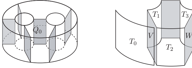
FIGURE 4.7. Left: the product bundle Q \times I for a pair of pants Q . Right: the prism Q_0 \times I .
