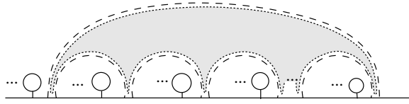
FIGURE 3.5. If \gamma runs over a sequence of non-prime arcs, then \gamma bounds a region (shown shaded above) containing no state circles, giving contradiction. Compare with Figure 2.8.
