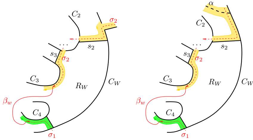
FIGURE 4.4. The region R_W in the case that \sigma_2 does not immediately connect to \beta_w . Left: Initially \sigma_2 enters R_W by running upstream. Right: Initially \sigma_2 enters R_W along a non-prime arc. In both cases, \sigma_2 runs across a state circle C_2 and eventually re-enters R_W .
