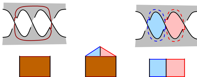
FIGURE 4.1. The EPD shown in the left side parabolically compresses to the EPDs shown in the right side.
