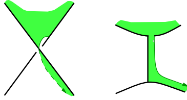
FIGURE 2.5. Left: A tentacle continues a shaded face in the upper 3–ball. Right: visualization of the tentacle on the graph H_A .
