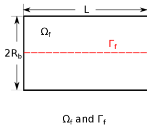
Figure 1.2: (left) A circular bilayer with interface \Gamma_{R_0} in a concentric domain of radius R_b . (right) A flat bilayer with interface \Gamma_f which intersects the rectangular domain at a right angle.
