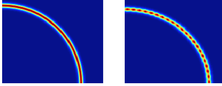
Figure 1.1: Quarter-plane views of equilibrium of the strong FCH equation (1.5) corresponding to radially symmetric bilayer initial data with \varepsilon = 0.1 and double well potential W as given in Section 5 of [6]. (left) For \eta_1 = 1 and \eta_2 = 2 , we have \alpha_0 < 0 , and the t = 3000 evolution is a circular bilayer equilibrium. (right) For \eta_1 = 2 and \eta_2 = 2 , we have \alpha_0 > 0 , and the t = 500 evolution of the initial data yields a circular pearly bilayer.
