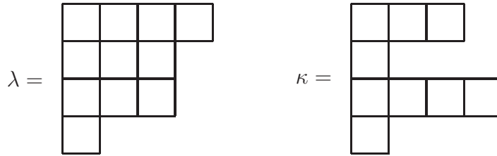
Figure 1: Ferrers diagrams for the partition \lambda = (4, 3, 3, 1) and the composition \kappa = (3, 1, 4, 1)
