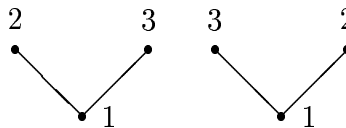
Two ordered trees
