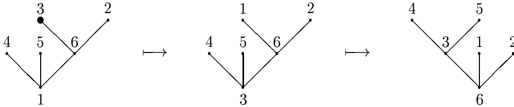
The bijection with l = 3 and r = 6
