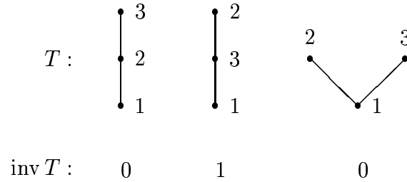
Trees and inversions for n = 3
