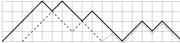
Fig. 2. The decomposition of Dyck paths.
