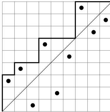
Fig. 3. The bijection \Gamma .
