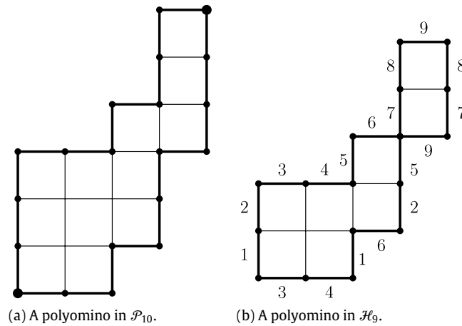
Fig. 5. Parallelogram and shortened polyominoes.
