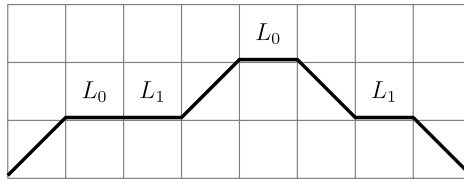
Fig. 1. The Motzkin path associated with \sigma = 361782495 .
