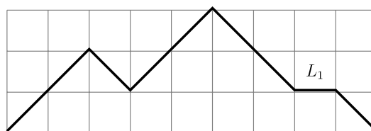
Fig. 6. The Motzkin path v(\sigma) associated with \sigma = 361782495 .
