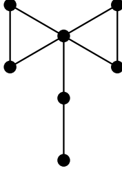
Figure 3: The exceptional graph E
