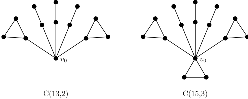
Figure 2: Examples of C(n, r) for n \geq 3r
