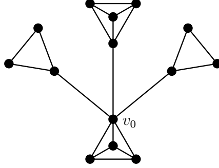
Figure 1: The graph C(14)
