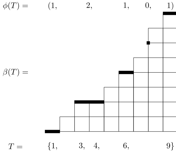
Fig. 4. The compositions \beta(T) and \phi(T) when n = 9 and T = \{1, 3, 4, 6, 9\} .
