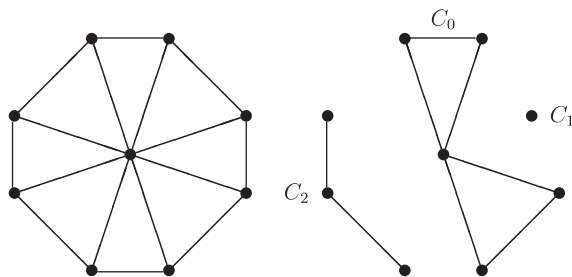
Fig. 3. The wheel W_8 a spanning tree, and components.
