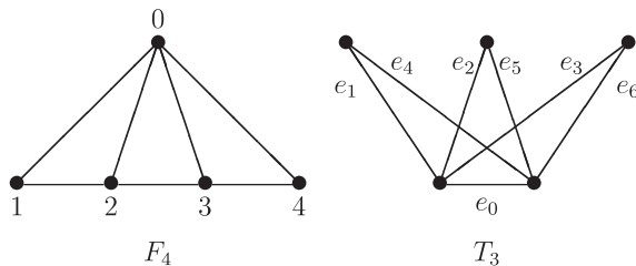
Fig. 2. The fan F_4 and triangle graph T_3 .
