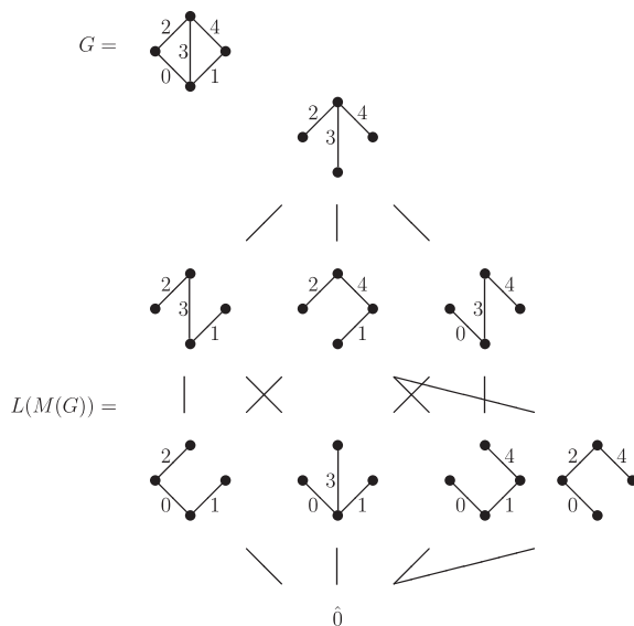
Fig. 1. An example graph and its external lattice.
