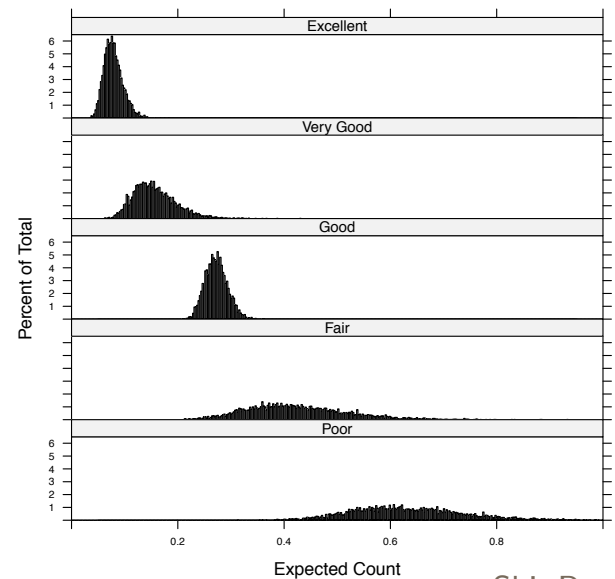
Elliptical Copula NB-II
